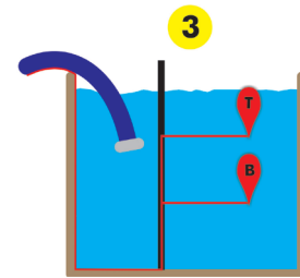
Water level causes both top and bottom float switches to rise. Engine automatically shuts down and the pump goes into Standby mode.
