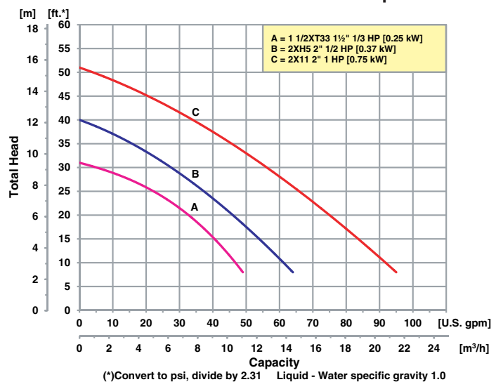
Performance of Submersible Pumps
